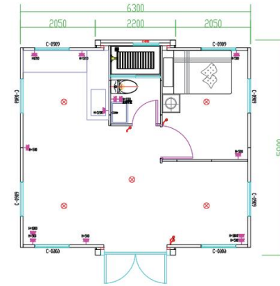
A 20ft One bedroom One bathroom
