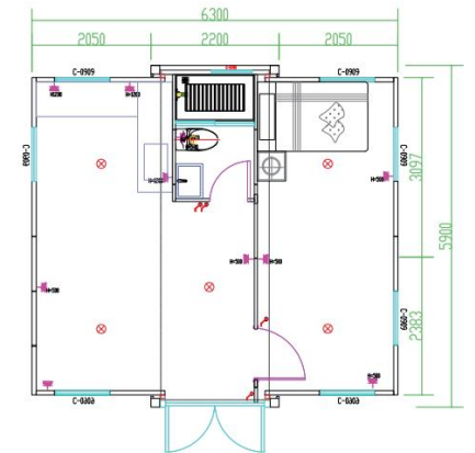
B 20ft One bedroom One bathroom
