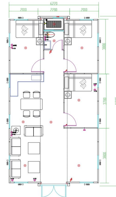
D 40ft Three bedroom One bathroom
