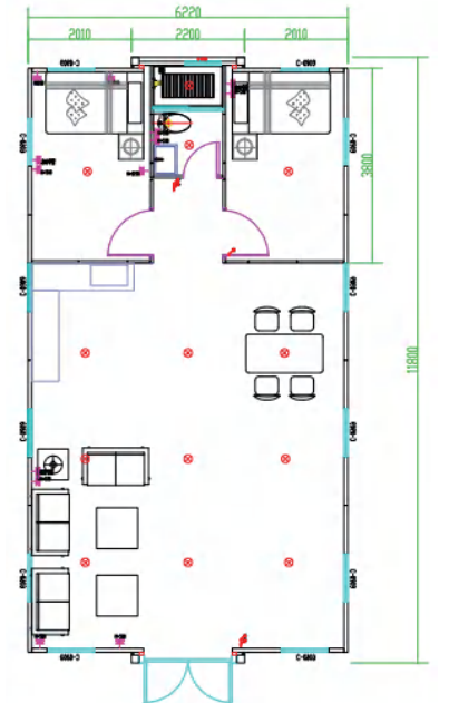
C 40ft Two bedroom One bathroom
