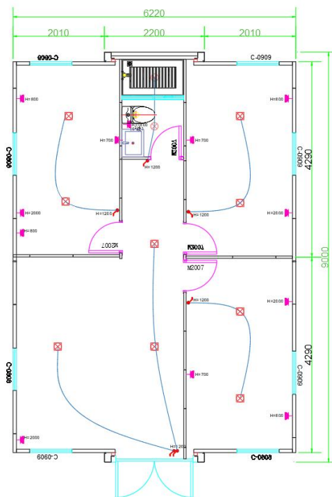
C 30ft Three bedroom One bathroom
