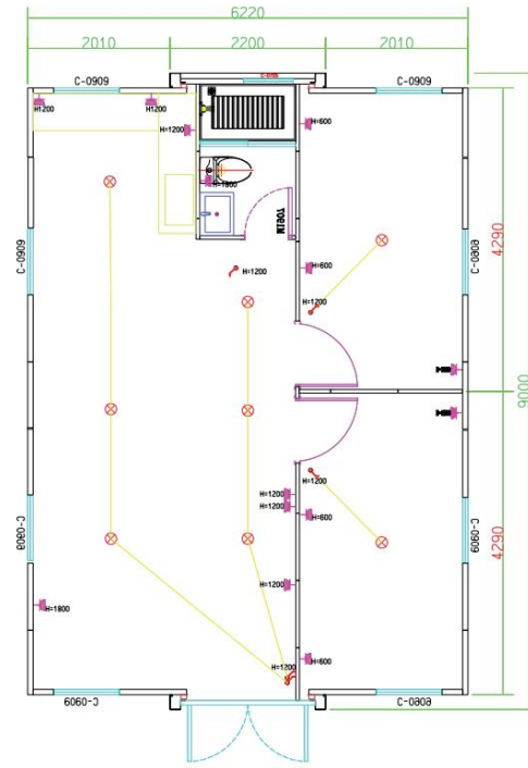
B 30ft Two bedroom One bathroom
