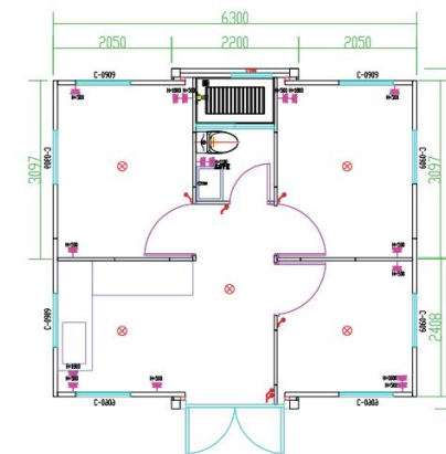
E 20ft Three bedroom One bathroom
