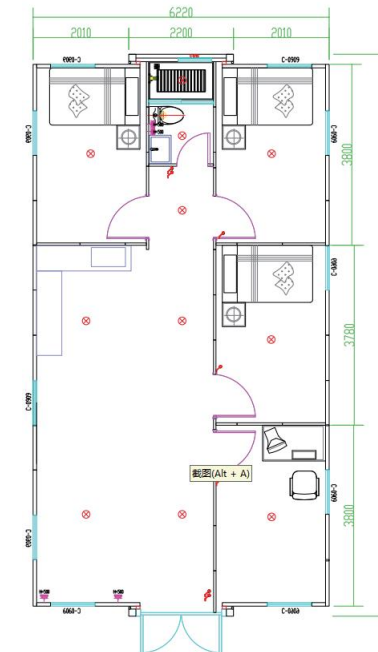
E 40ft Four bedroom One bathroom
