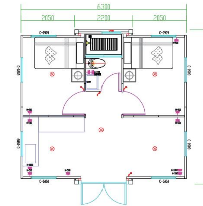
C 20ft Two bedroom One bathroom
