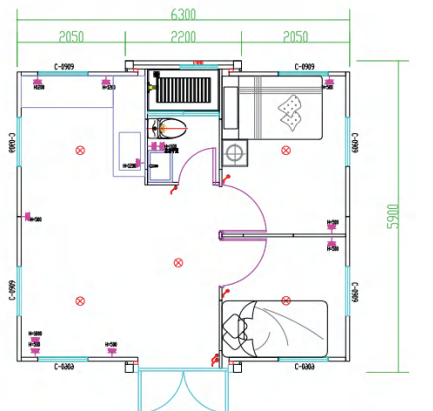
D 20ft Two bedroom One bathroom
