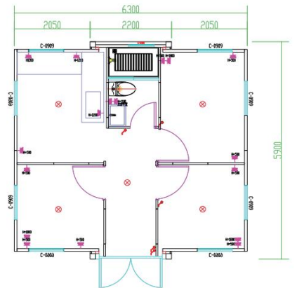
F 20ft Three bedroom One bathroom
