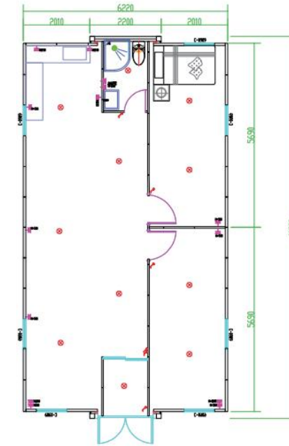
A 40ft Two bedroom One bathroom
