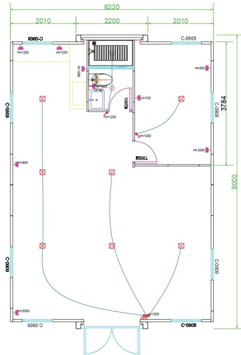
A 30ft One bedroom One bathroom
