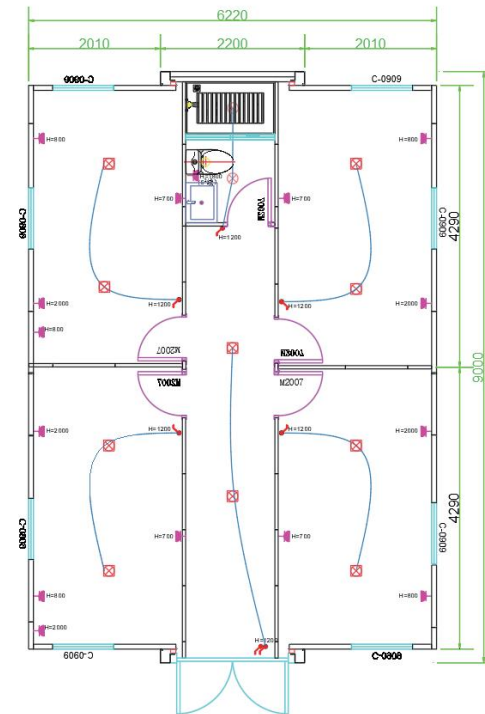
D 30ft Four bedroom One bathroom
